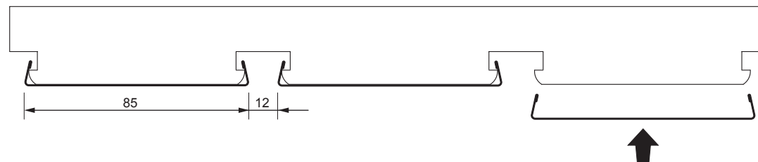
Instalación TA-85 Installation TA-85 Installation TA-85
